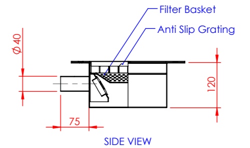
General Gully 200 x 200mm Side outlet Ø40mm
